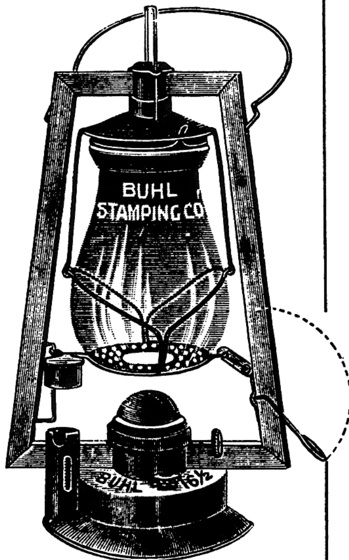
No. 16½ Showing Globe Raised. Patented March 30, 1897. Patents Applied For.
